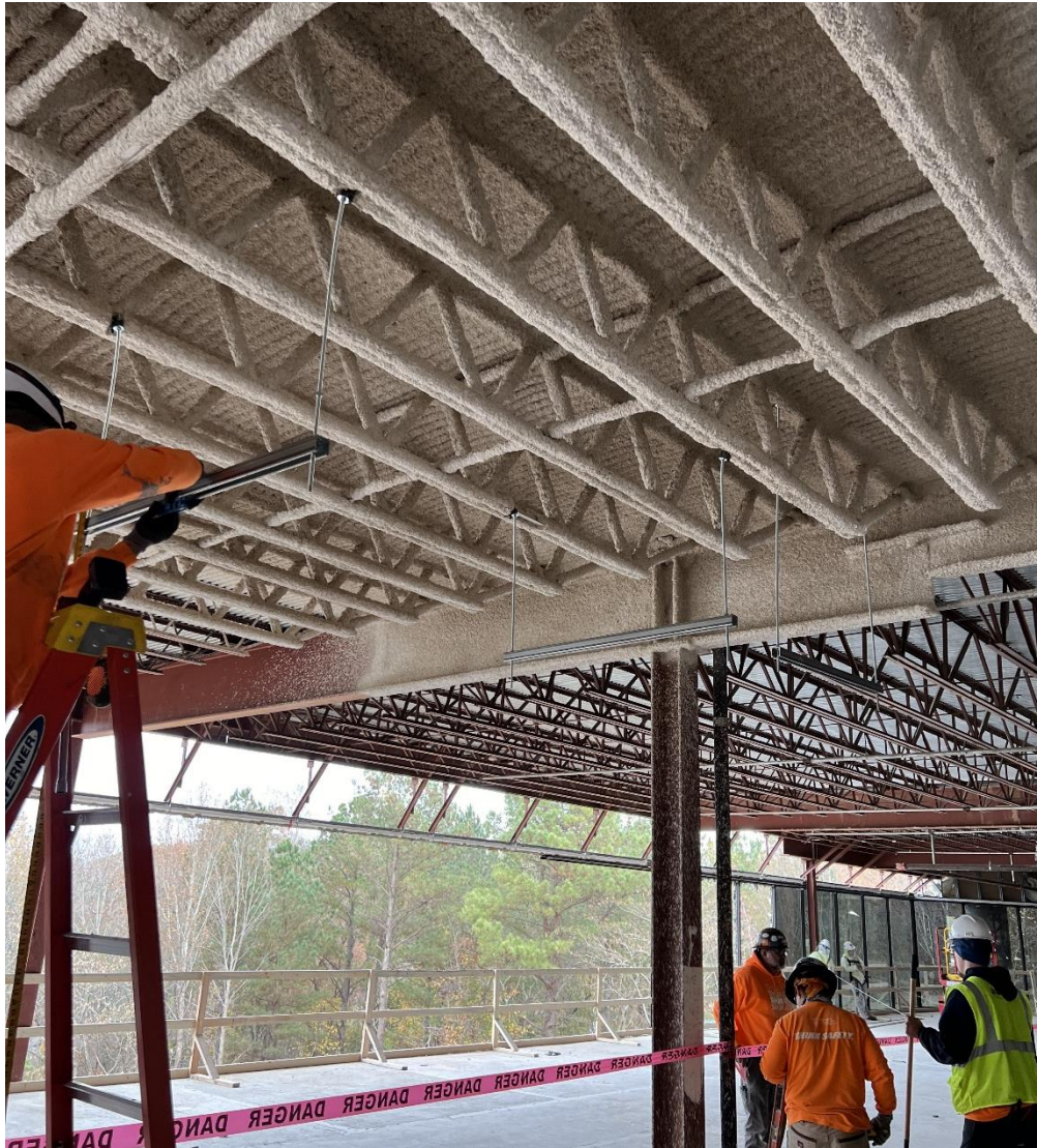
Mechanical Overhead Rough-in On Level 2
