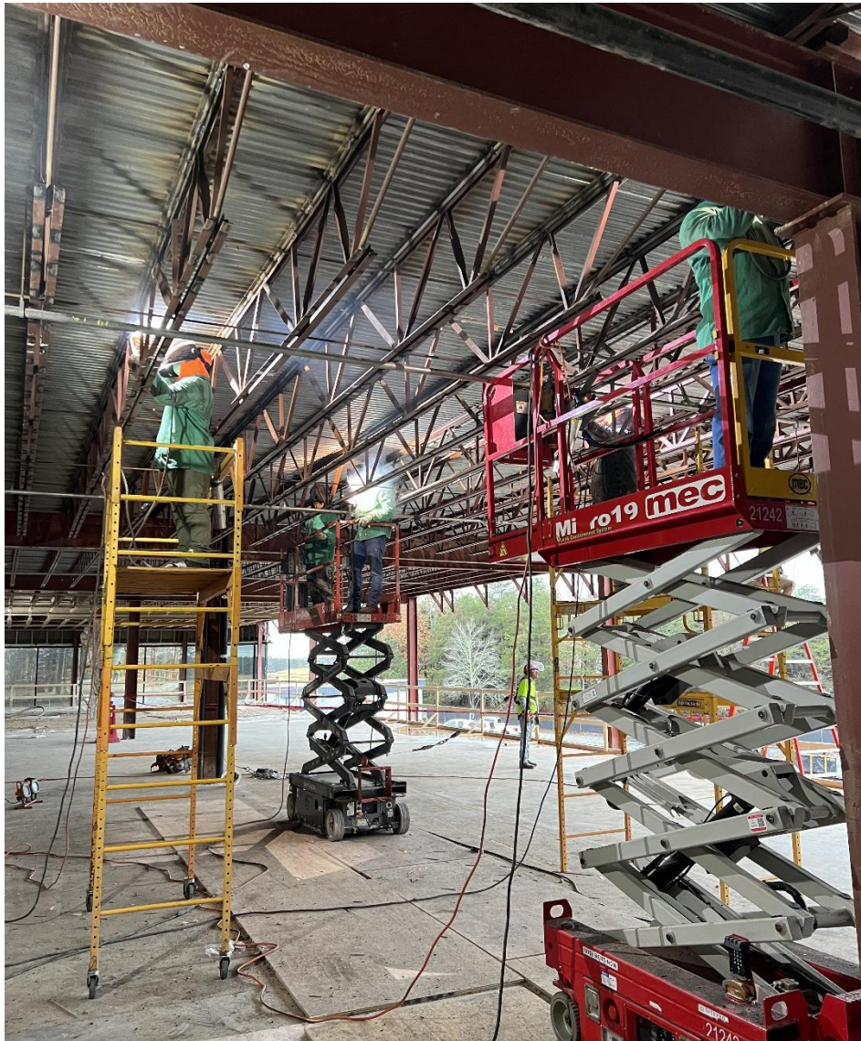
Continue joist augmentation on level 1
