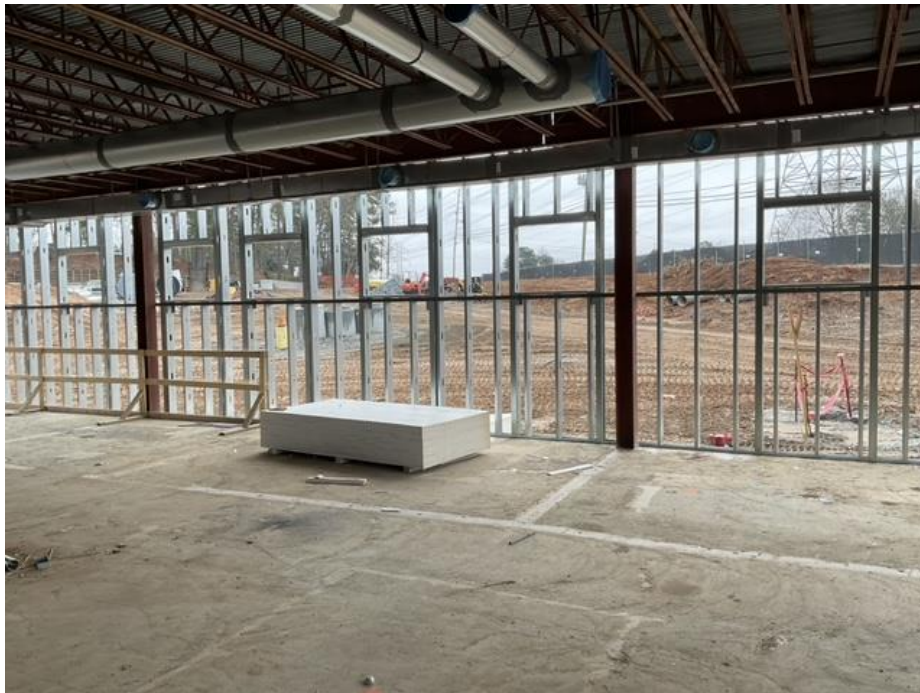
Exterior Framing
