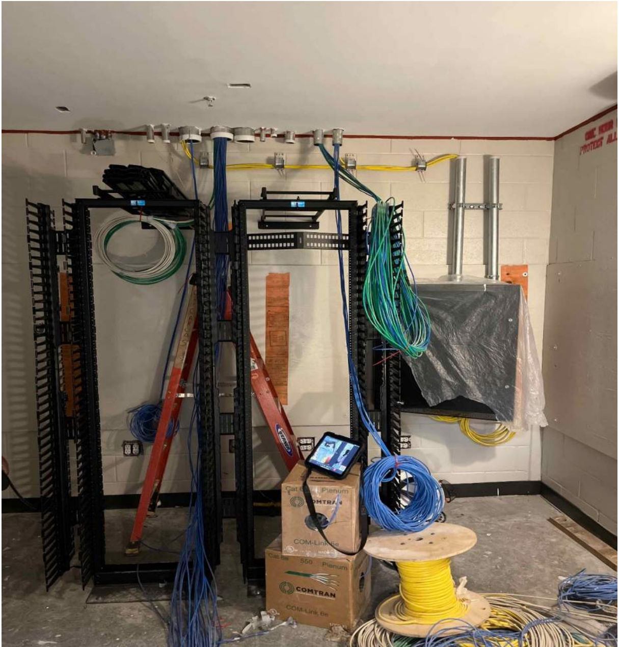
Installation of Data Rack at Second Floor Data Room
