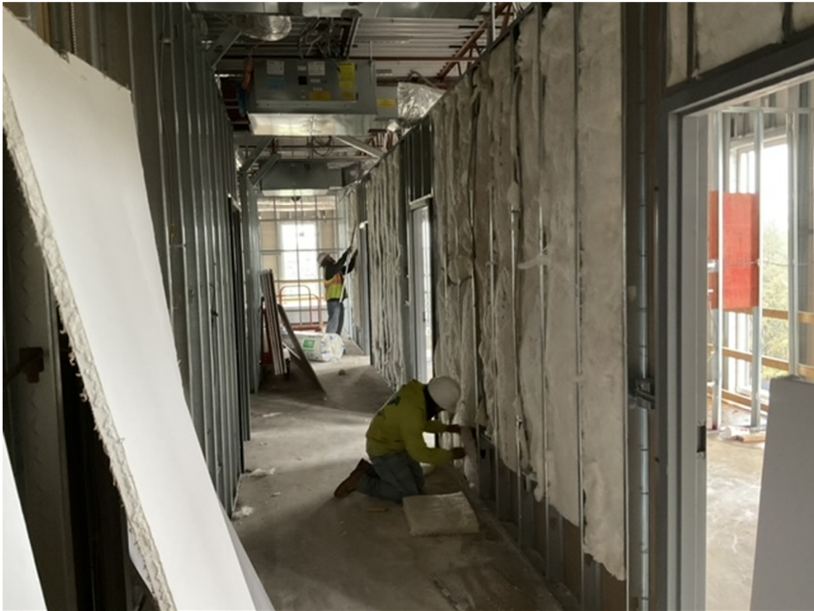
Sheetrock/Insulation Installation
