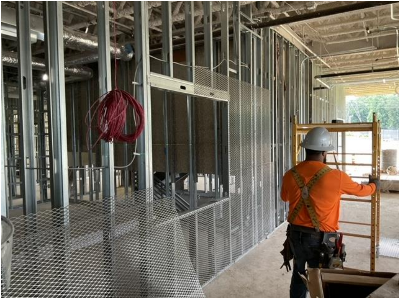
Interior framing/ security mesh
