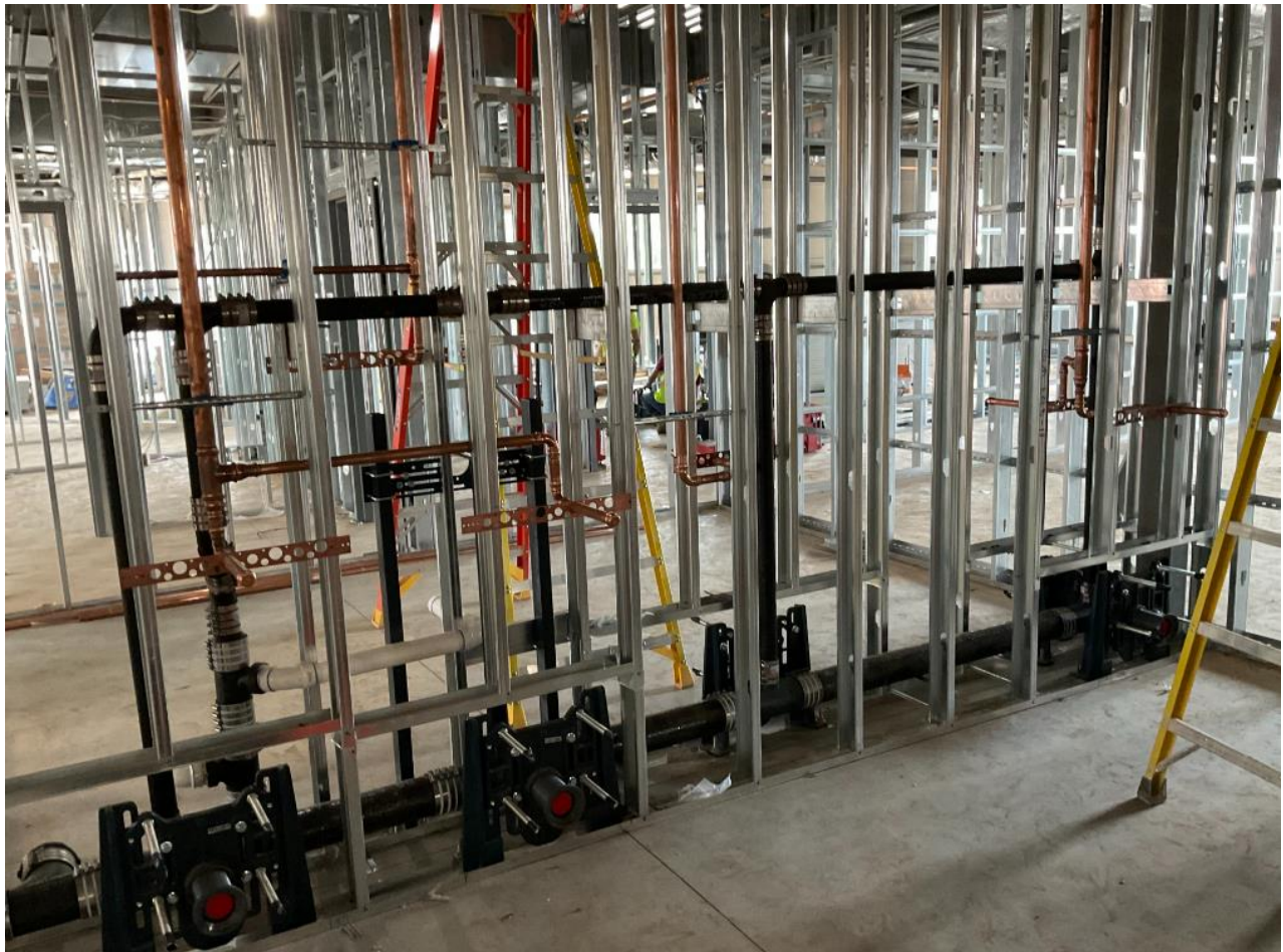
Framing & MEP Rough-In at Courts Addition Restrooms
