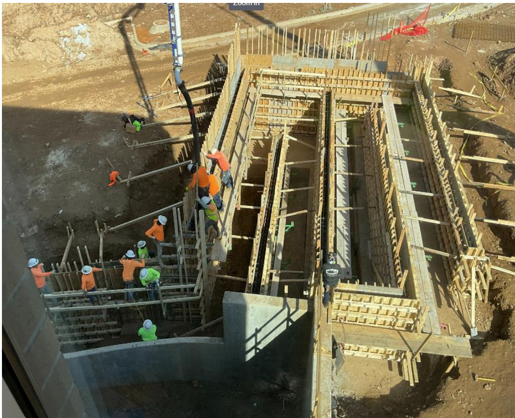
Formwork for Wall B Walls
